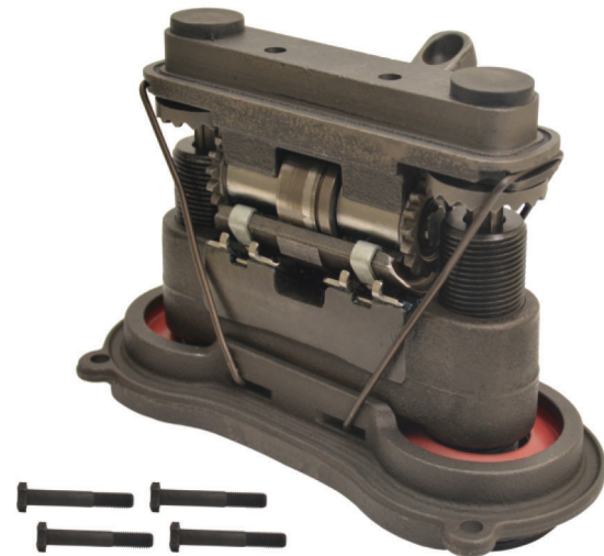
COMPLETE MECHANISM SET
